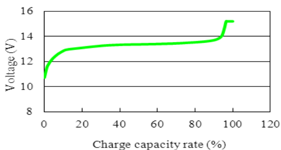
Charge characteristic
