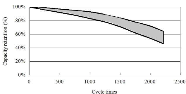
Cycle life
